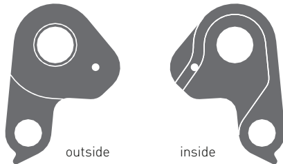
Hanger for SRAM & Shimano Standard
